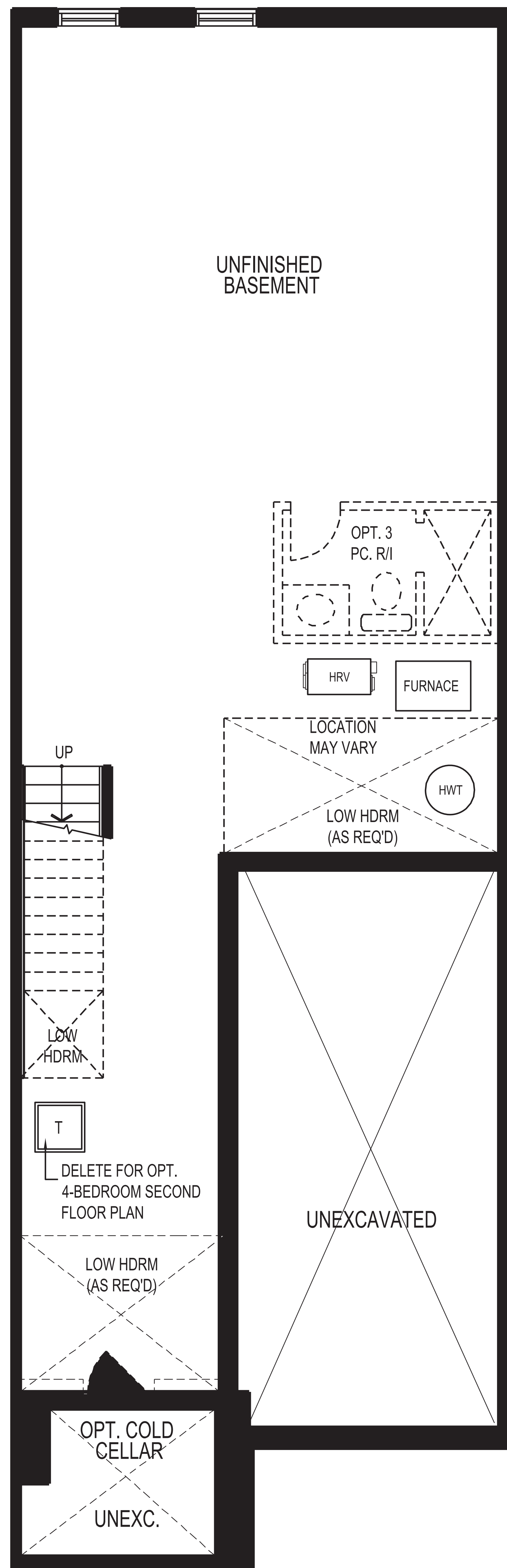
BASEMENT PLAN ELEV. 'A1', 'A2', 'B1', 'B2'
