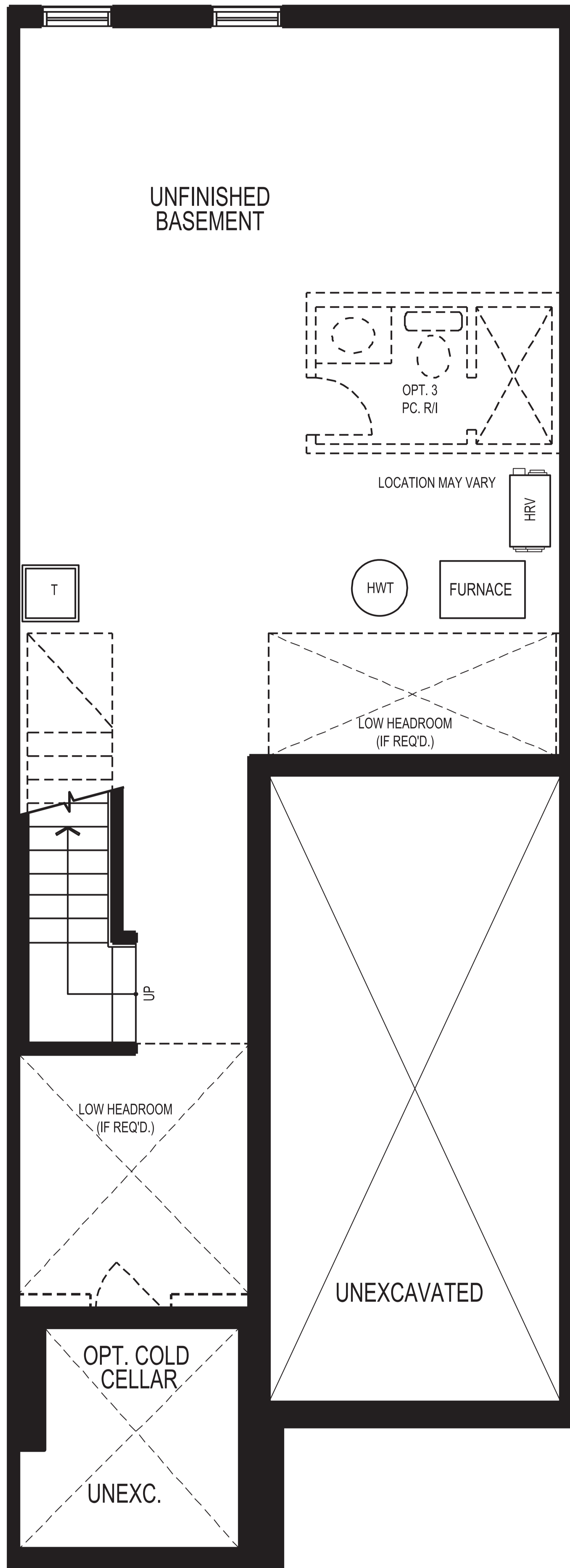
BASEMENT PLAN ELEV. 'A1', 'A2', 'B1', 'B2'
