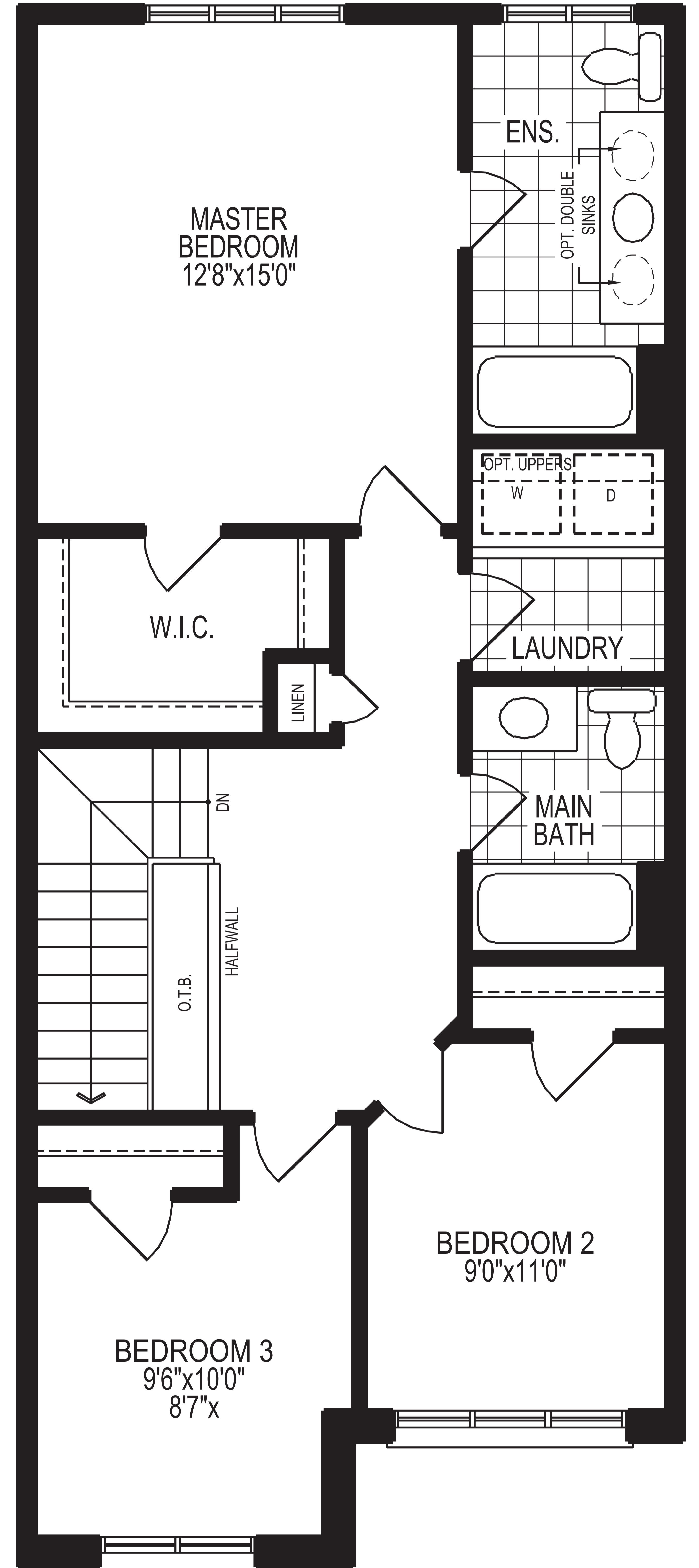
SECOND FLOOR PLAN, ELEV. 'A1'
