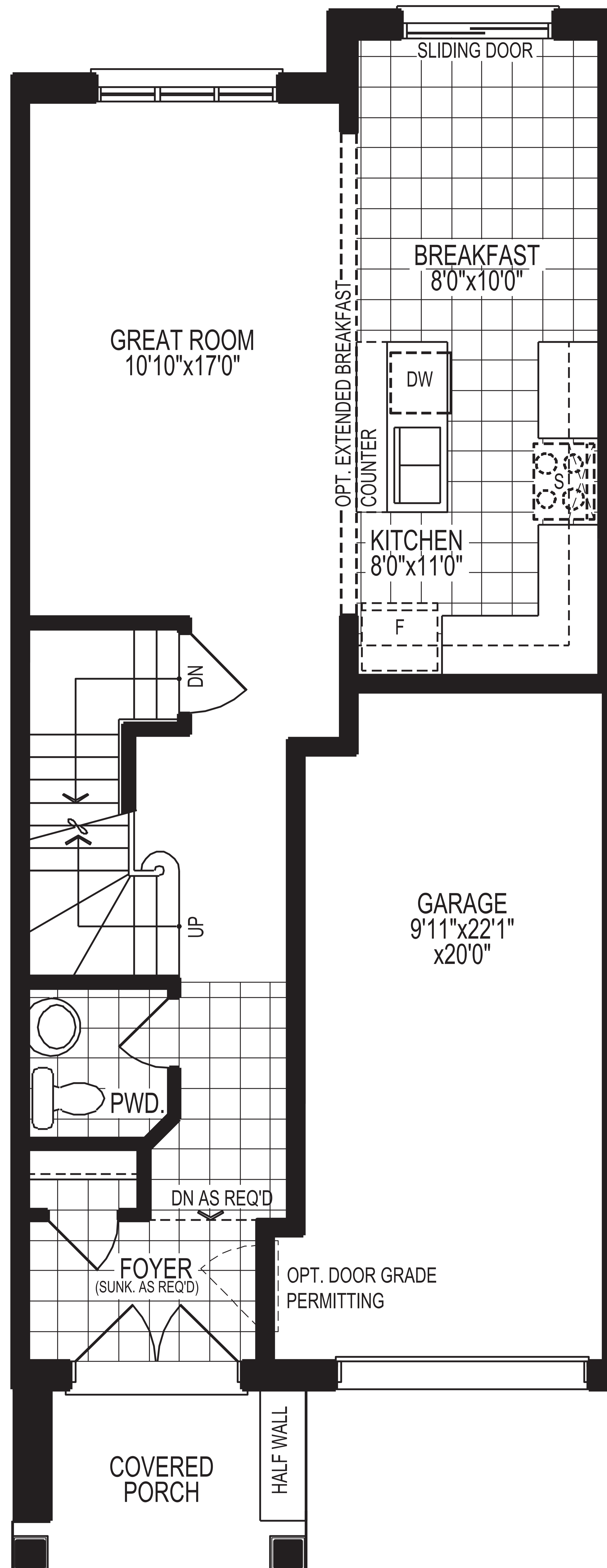
GROUND FLOOR PLAN, ELEV. 'A1' & 'A2'
