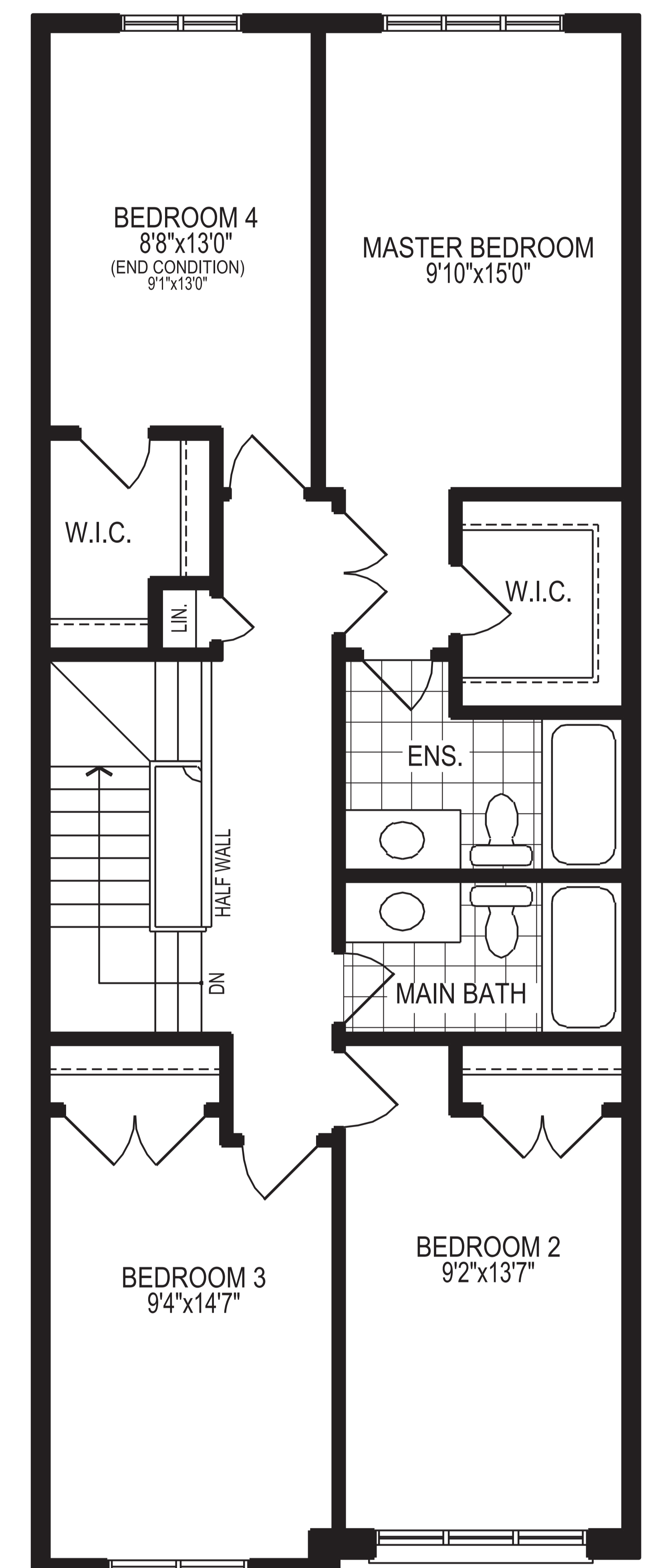
OPT. 4-BEDROOM SECOND FLOOR PLAN, ELEV. 'A1' ('A2', 'B1' & 'B2' SIMILAR)
