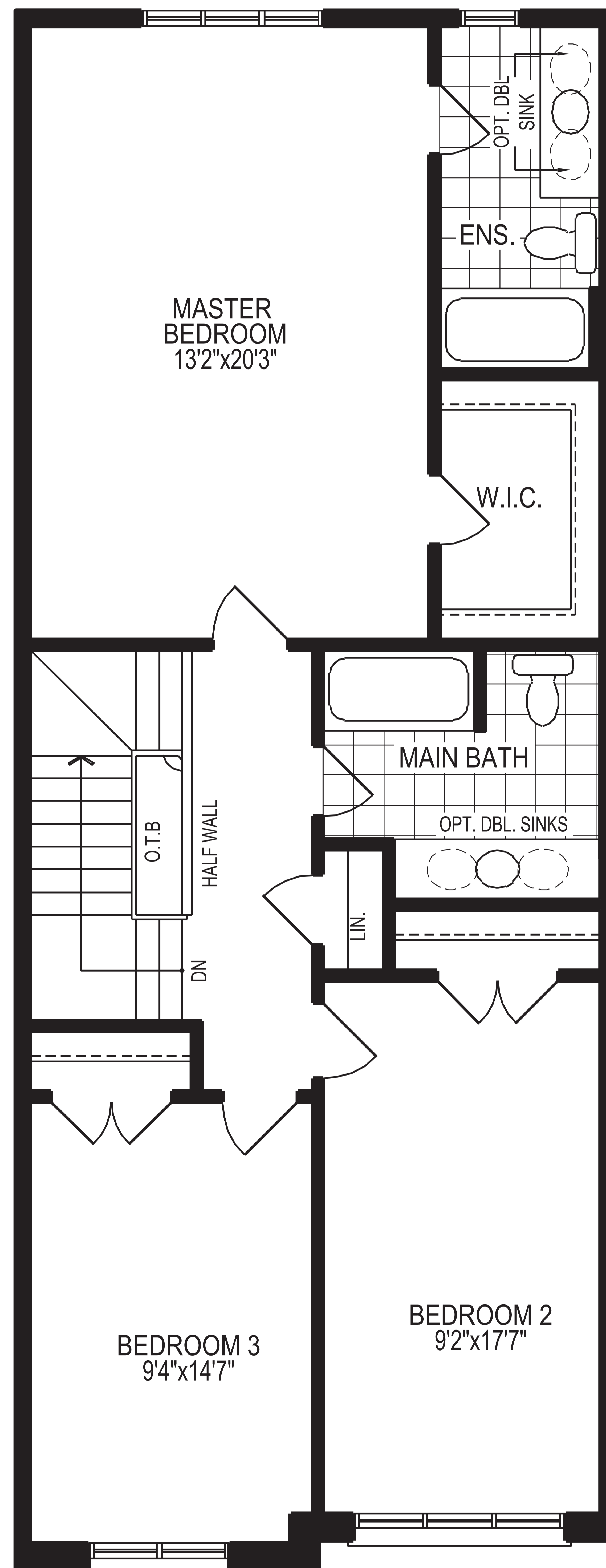
SECOND FLOOR PLAN, ELEV. 'A1'
