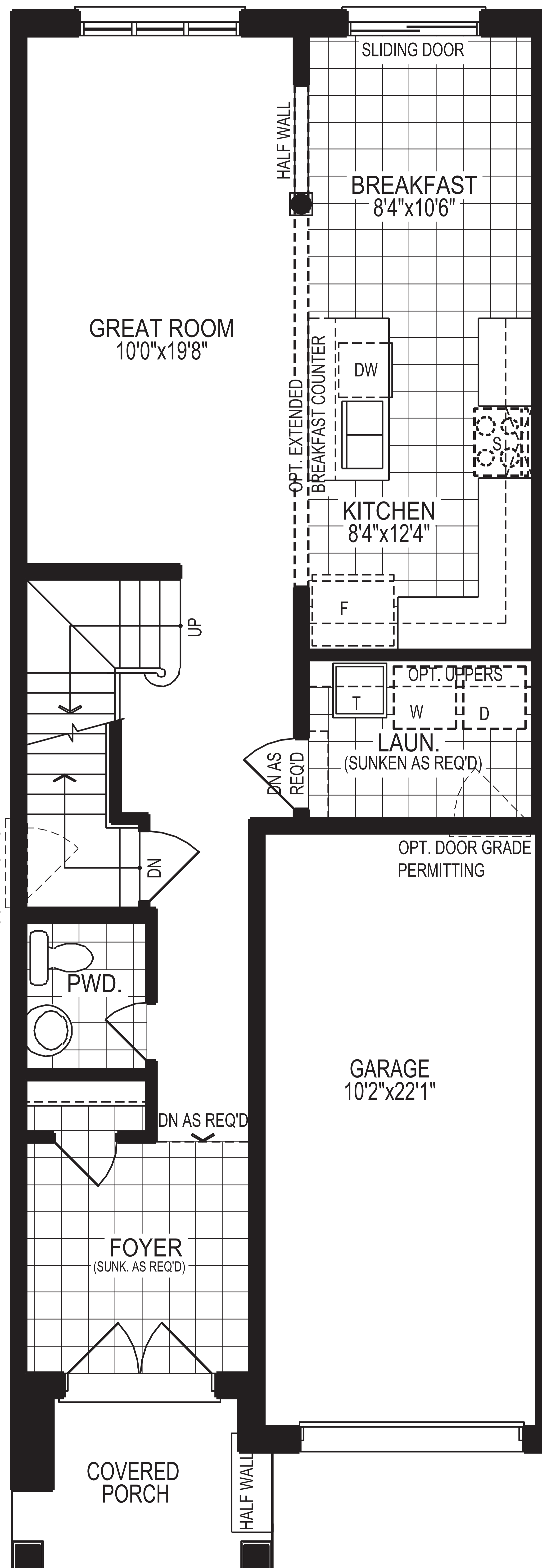
GROUND FLOOR PLAN, ELEV. 'A1' & 'A2'
